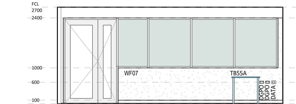
2 ELEVATION DETAIL 60-033 1 : 50
