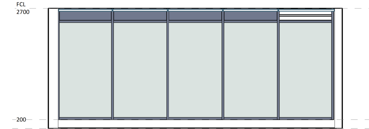
4 ELEVATION DETAIL 60-033 1 : 50
